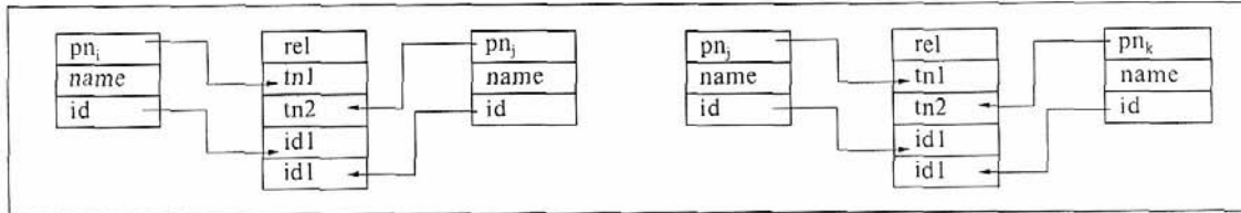
Figure 5. The relationship p between tables (where i < j < k )
